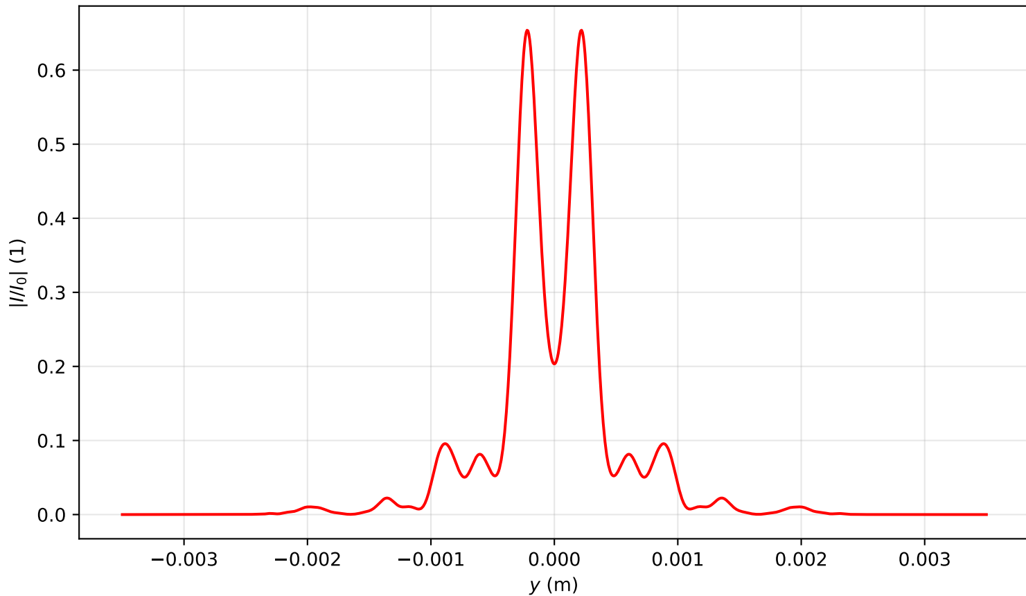
Intensity profile I(x = 0, y, z = 1.672)/I_0 , P_{in}=6.0P_{cr} , artificial time
